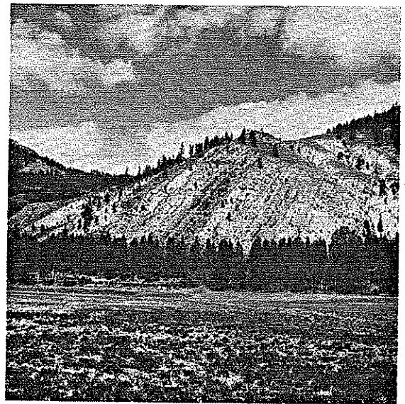
FIGURE 11.—Winthrop Sandstone. Upper part of type section truncated by Boesel Fault. Outcrop northeast side of State Highway 20, 6 miles northwest of Winthrop
