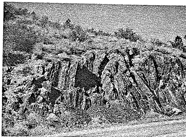
FIGURE 3.—Twisp Formation. Folded black shales 1.8 miles south of Winthrop on State Highway 20.
