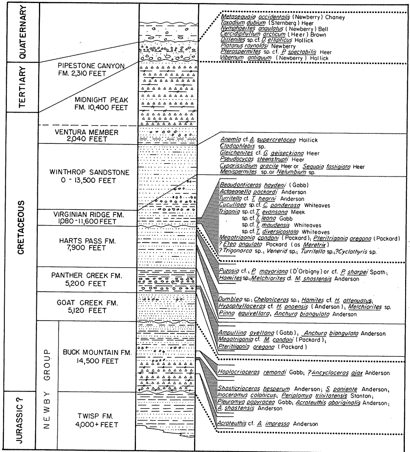
FIGURE 14.—Paleontologic section, Methow Valley.
