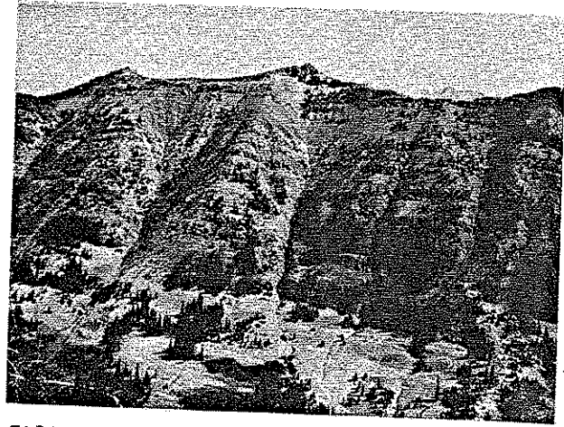
FIGURE 10.—Virginian Ridge Formation. Predominantly black shale, with chert pebble conglomerate and chert grain sandstone making hard outcrop. View to the northeast (Robinson Mountain in distance). Road in lower left is 2.5 miles southeast of Harts Pass.
