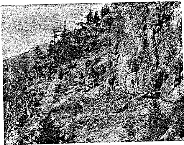
FIGURE 17.—Thrust fault, Midnight Peak Formation, Volcanic (upper) Member over older Ventura Member red beds. Face of spur between Lost River and Robinson Creek, Methow Valley.
