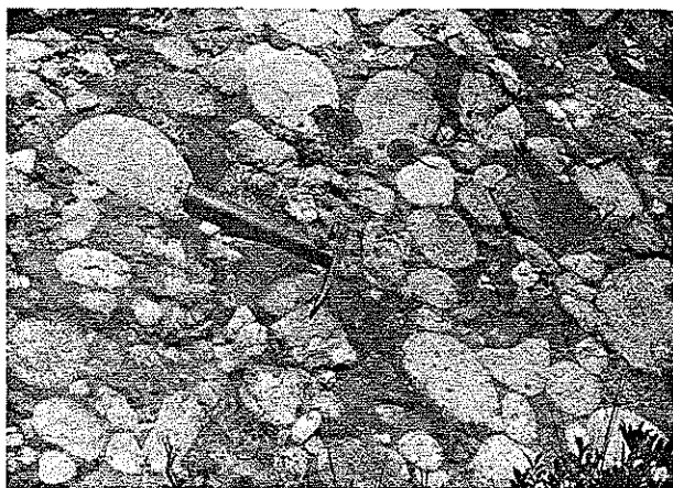
FIGURE 6.—Panther Creek Formation. Glacially eroded, horizontal surface on near-vertical bed of granitoid cobble-boulder conglomerate from type section.
