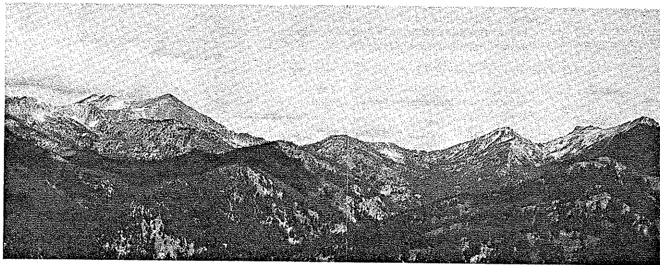
FIGURE 5.—Looking north-northwest from Sweetgrass Butte showing type sections of Goat Creek and Panther Creek Formations.
