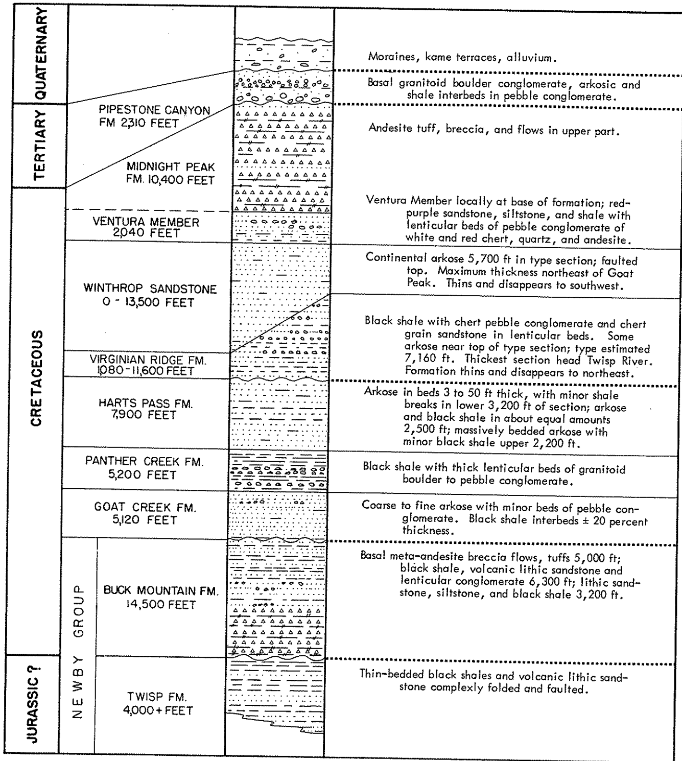
FIGURE 15.—Stratigraphic section, Methow Valley.
