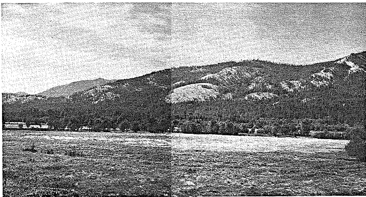
FIGURE 9.—Type section Virginian Ridge Formation. Photo looking southwest from State Highway 20, 5 miles west of Winthrop.
