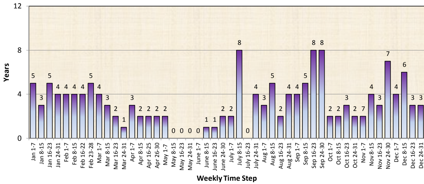
Number of Occurrences of 7-Day Periods below Minimum Flows on the Chewuch River at Winthrop WA, by Weekly Time Steps for the 1991-2015 Period of Record
