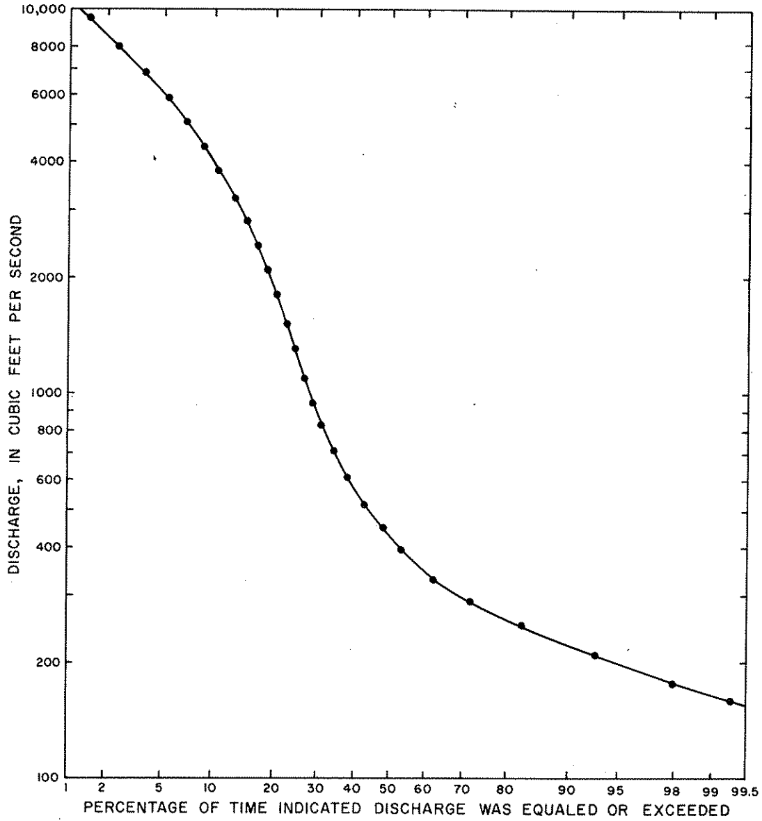
FIGURE B8. Flow-duration curve for the Methow River at Twisp (12449500), for the period June 1919-September 1962.
