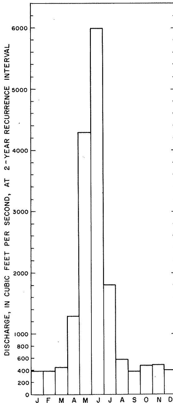
FIGURE B3. Frequency distribution of monthly mean discharge of Methow River near Pateros (12449650), for the period Oct. 1, 1958-Sept. 30, 1970.
