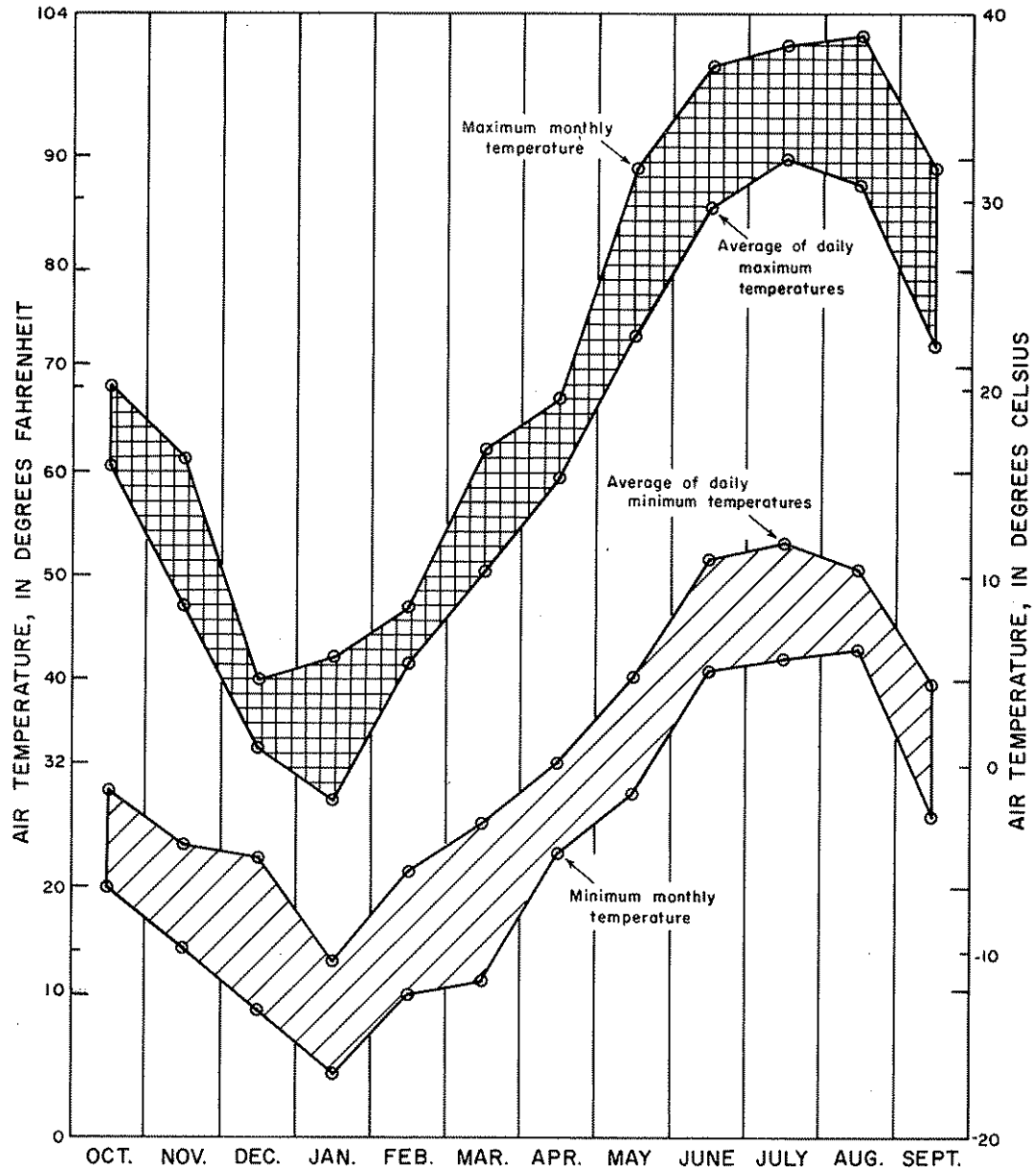
FIGURE A7. Trends in air temperature at U.S. Weather Service station at Methow, during the period Oct. 1, 1969–Sept. 30, 1970.
